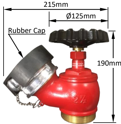
Hydrant Valve \varnothing 2\frac{1}{2}'' (DN65) Model HV005-1V-65
