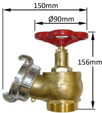
Hydrant Valve \varnothing 2'' (DN50) Model HV-005-1V-50
