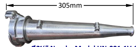
\varnothing 2\frac{1}{2}'' Nozzle, Model HN-001-1V-65
