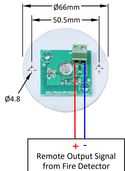
Typical Termination Diagram
