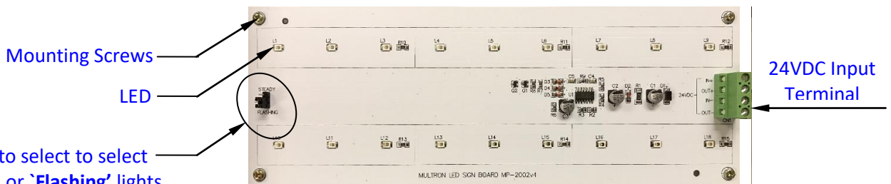
Typical LED Board within the Signage Cabinet
