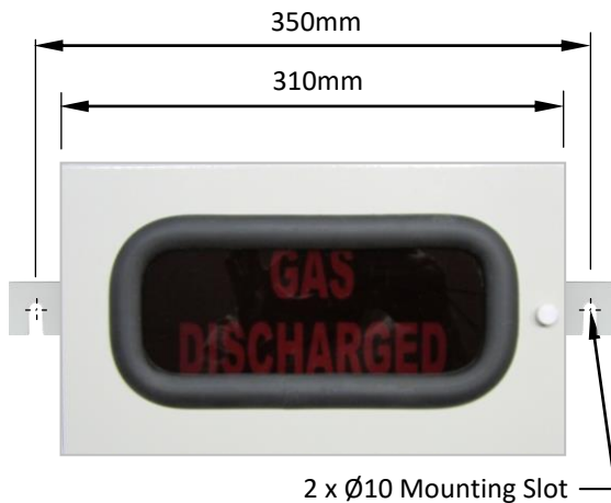
Typical Weatherproof Signage Model : GD-V4-W Model : EA-V4-W
