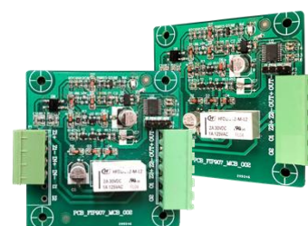
ISOLATOR MODULE (Optional), FIP907 (To be mounted within the RTTU Cabinet)
